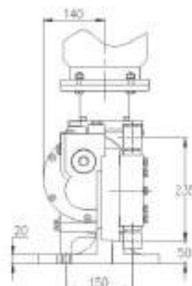
RX100-140 metal fluid end front view
