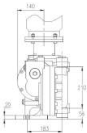
RX700-1200 metal fluid end front view
